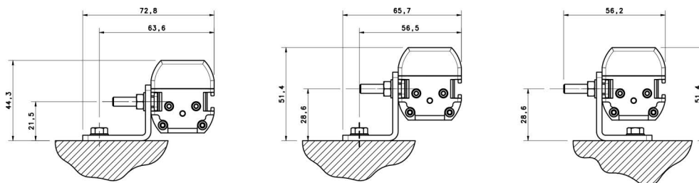
Figure 60 - Angled fixing bracket
