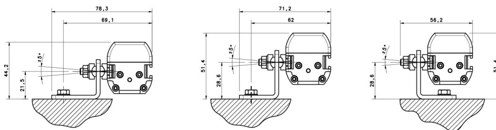
Figure 61 - Angled fixing bracket + Orientable support
