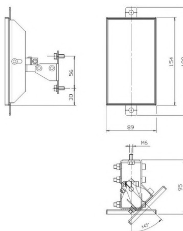
Figure 73 - SG-DM 150 (mm)
