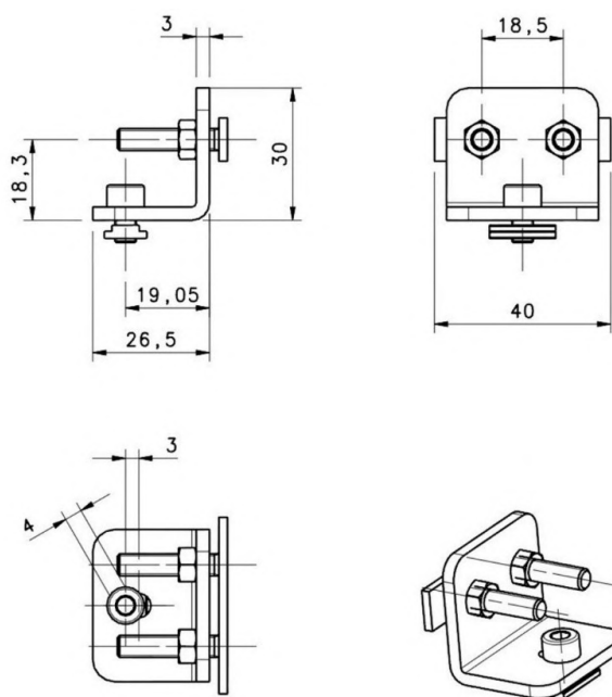
Figure 68 - Mounting kit
