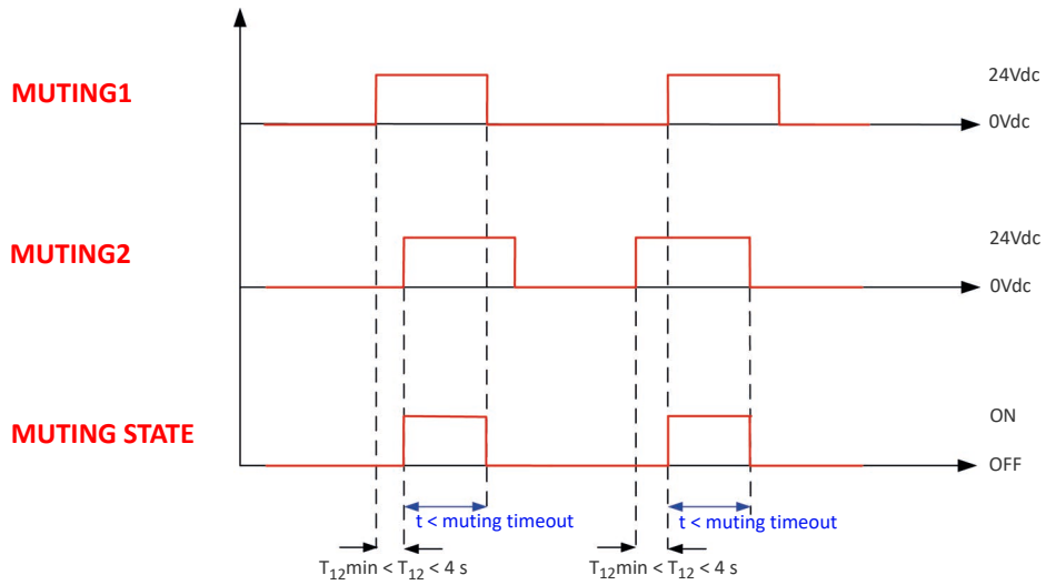
Figure 43: T muting timings
