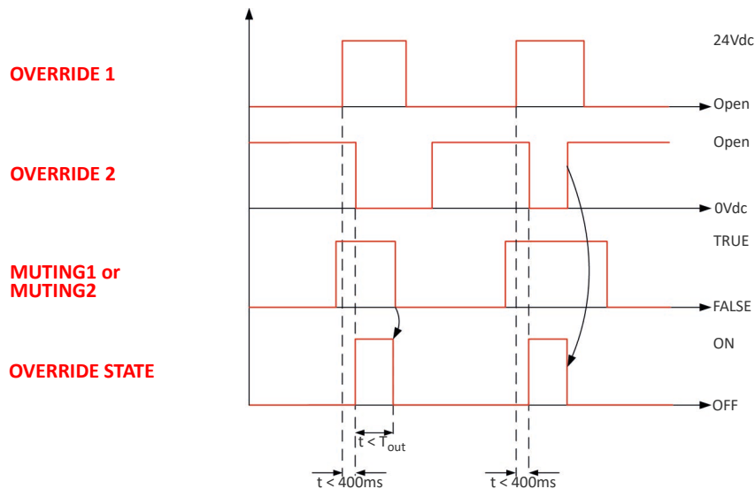
Figure 48: Level Triggered Override Timings
