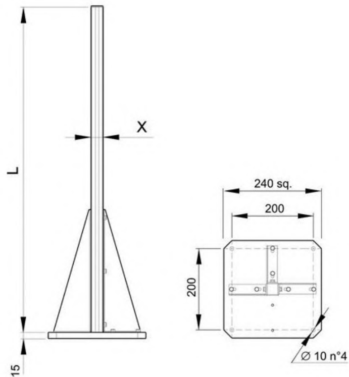
Figure 71 - Dimensions (mm)
