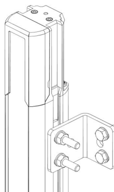
Figure 20: Fixing with two screws
