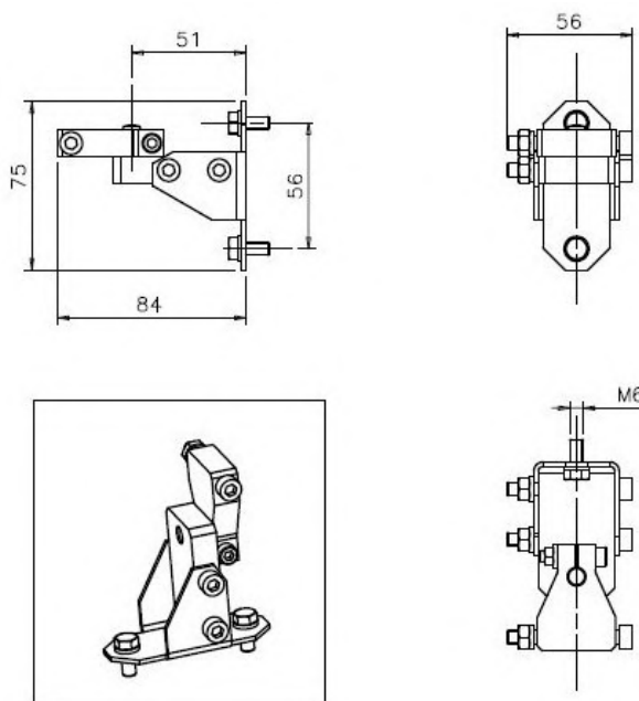
Figure 74 - Mounting kit
