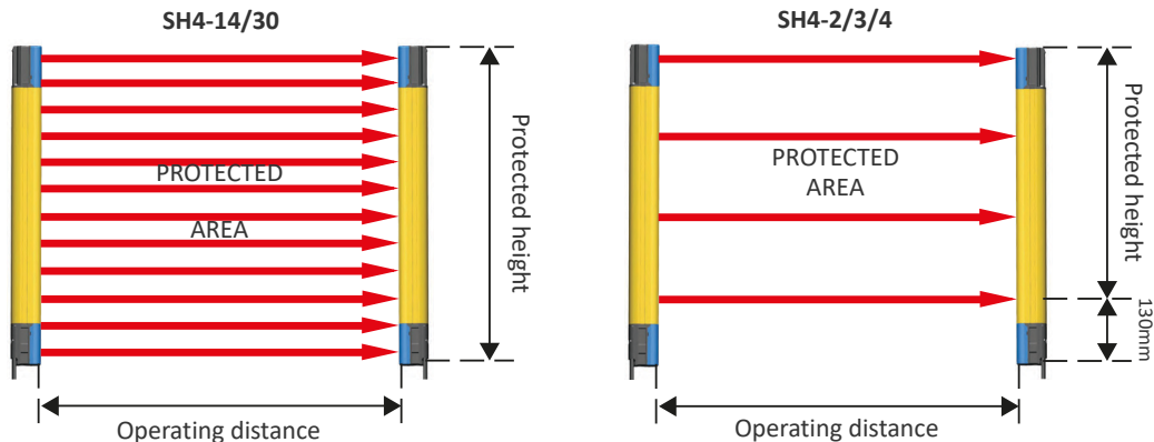
Figure 2: Detection zone
