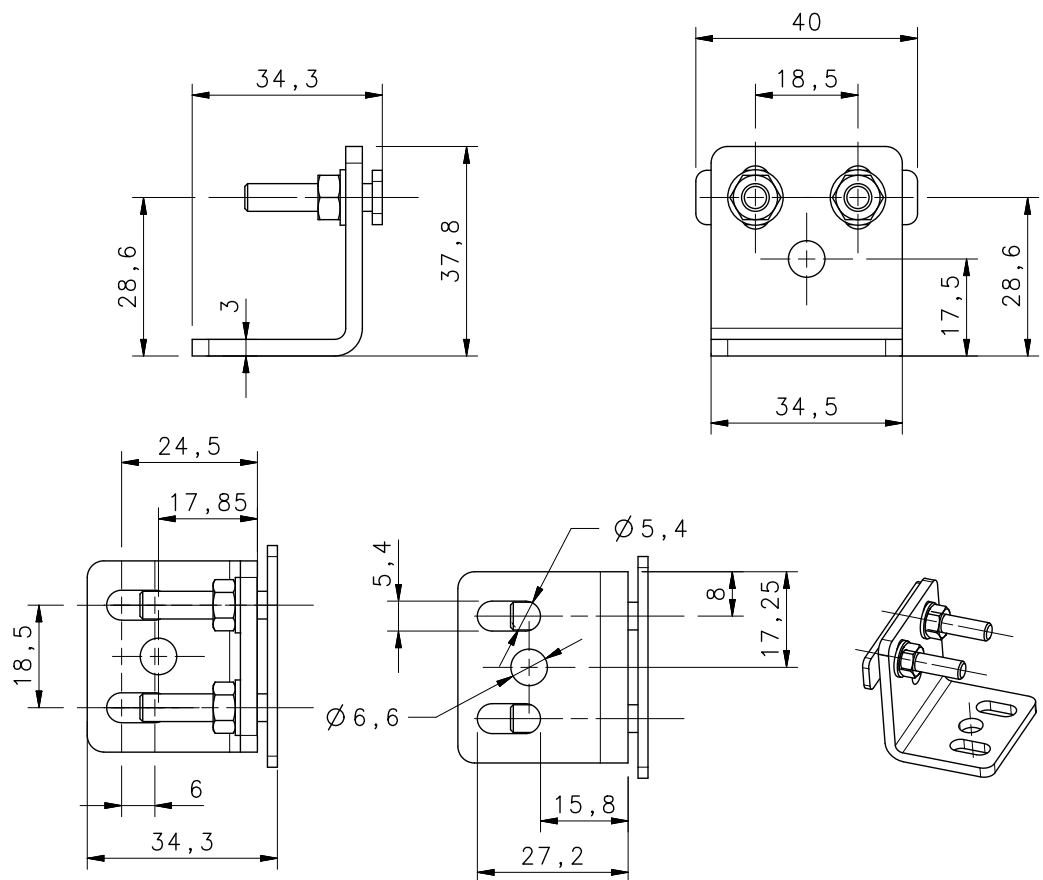
Figure 59 - ST-KSTD
