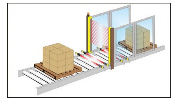
Figure 39: Linear version with external Muting sensors
