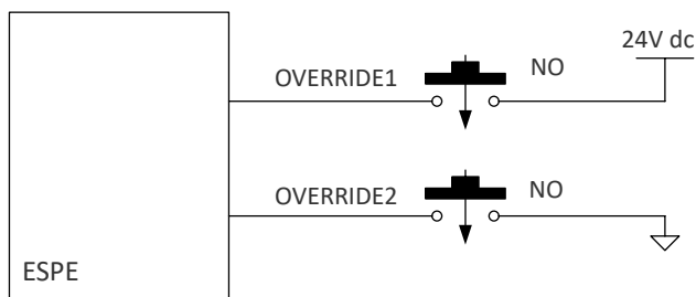
Figure 47: Override connection for SM-8-5 models
