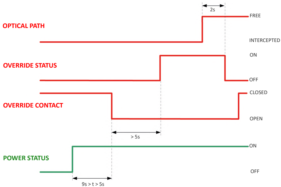
Figure 50: Override at startup timings
