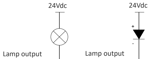
Figure 46: Muting Signaling Device connection
