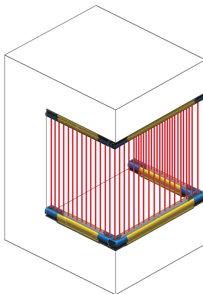
Figure 88: Application example
