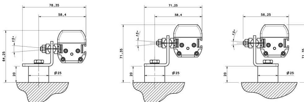
Figure 63 - Angled fixing bracket + Orientable support + Anti-vibration support
