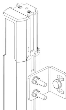
Figure 21: Fixing with a screw
