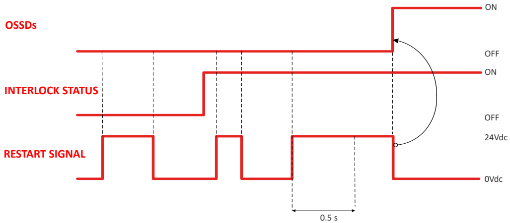
Figure 30: OSSDs behavior in Manual Restart Mode and Restart Pattern (SM-8-5)
