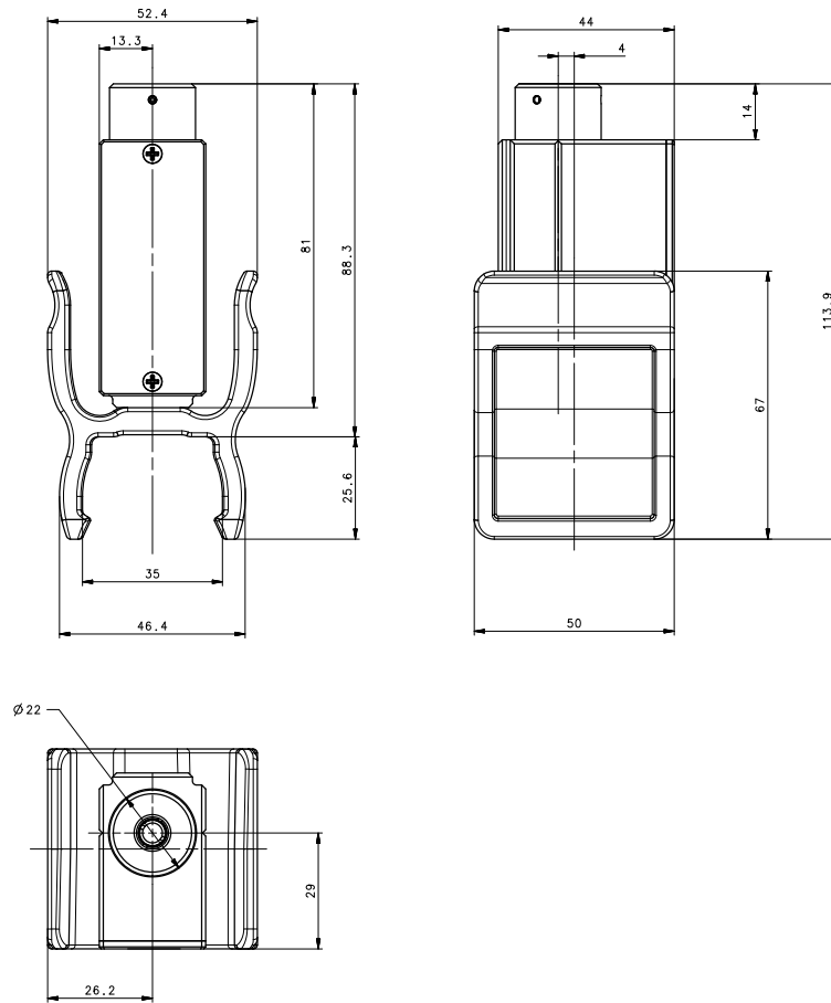
Figure 76 - Dimensions (mm)
