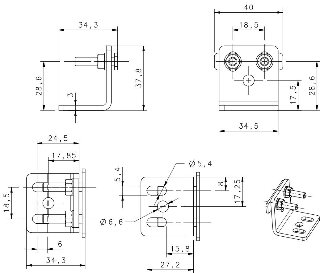
Figure 58 - Metal Angled fixing Bracket
