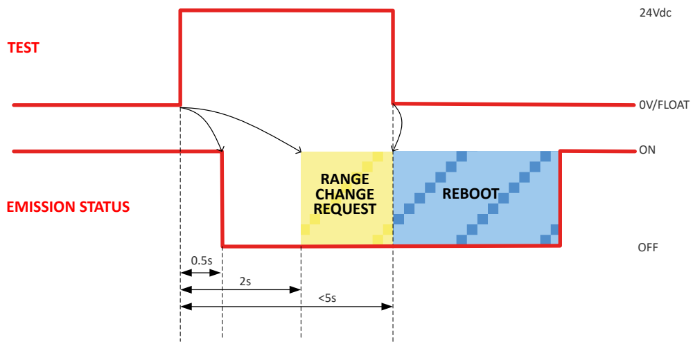
Figure 36 Emission Range Change Request timings
