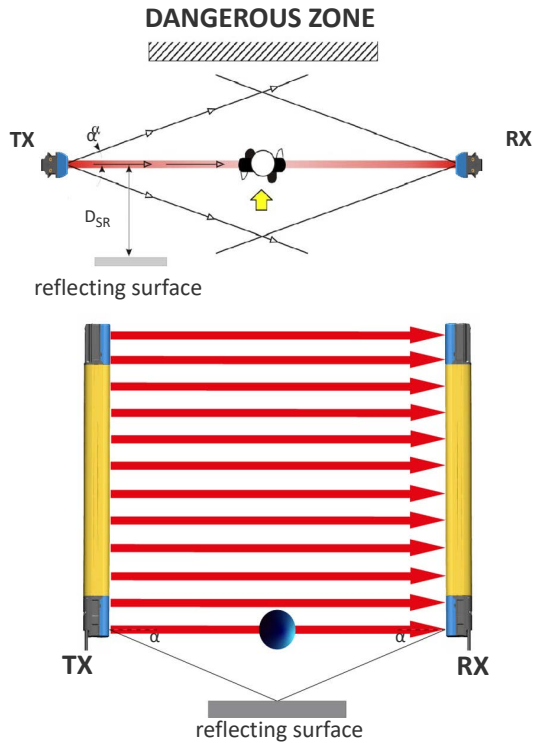
Figure 9: Distances from reflective surfaces
