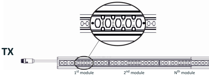
Figure 91: Transmitter LED interface
