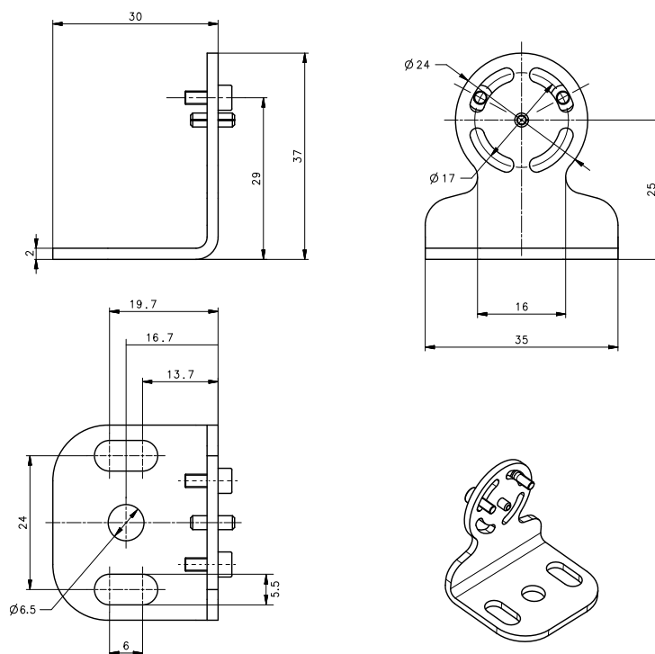
Figure 64 - ST-K4ROT-SH
