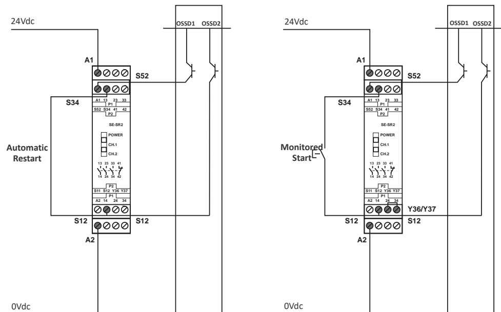
Figure 24: Connection to SE-SR2 Safety Relays
