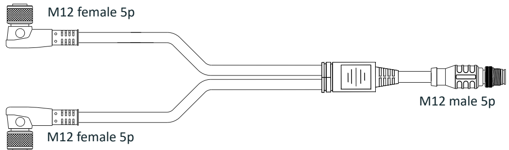
Figure 84: T muting cable
