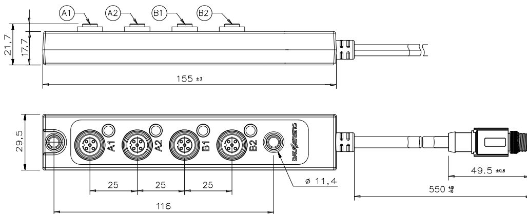
Figure 87 - Dimensions (mm)
