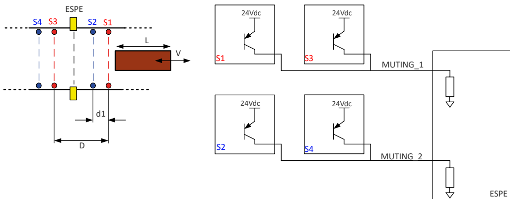
Figure 44: Connection of sensors on MUTING1 and MUTING2 inputs in case of bidirectional (T), four-sensors muting
