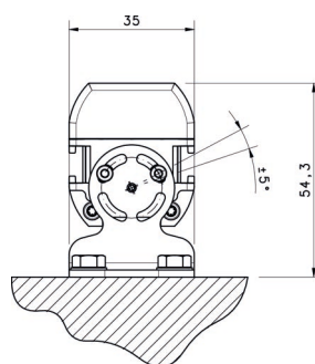
Figure 65 - Straight mounting
