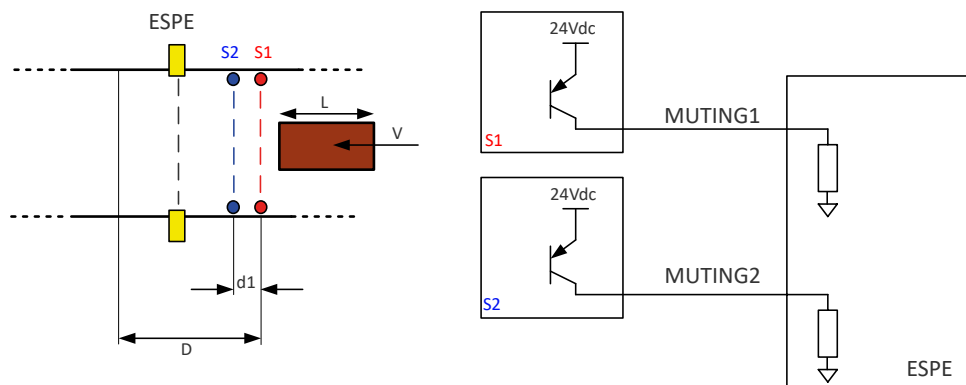
Figure 42: Connection of sensors on MUTING1 and MUTING2 inputs in case of monodirectional (L), two-sensors muting
