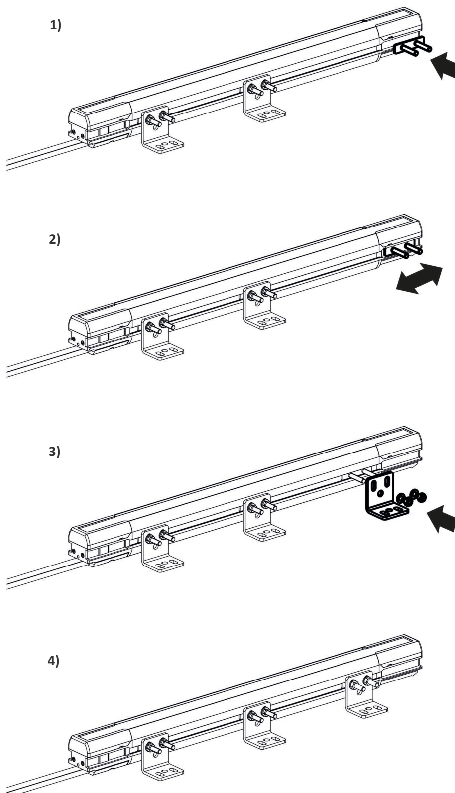
Figure 18: Fixed brackets mounting procedure
