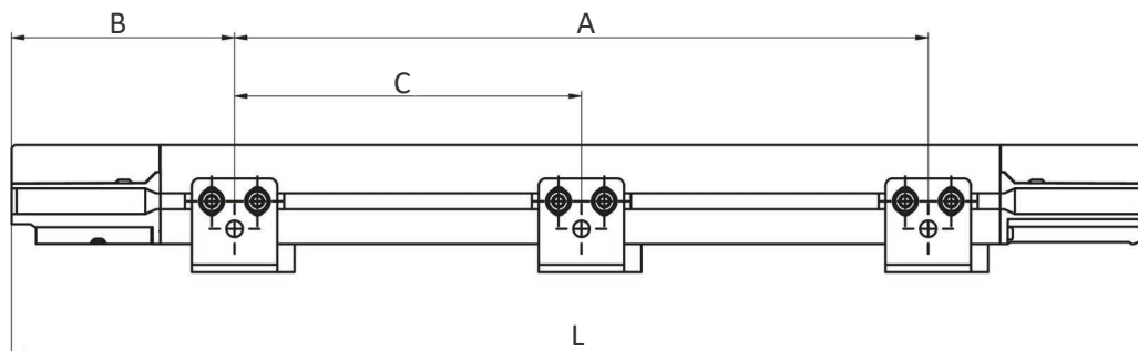
Figure 19 - Light curtain dimensions
