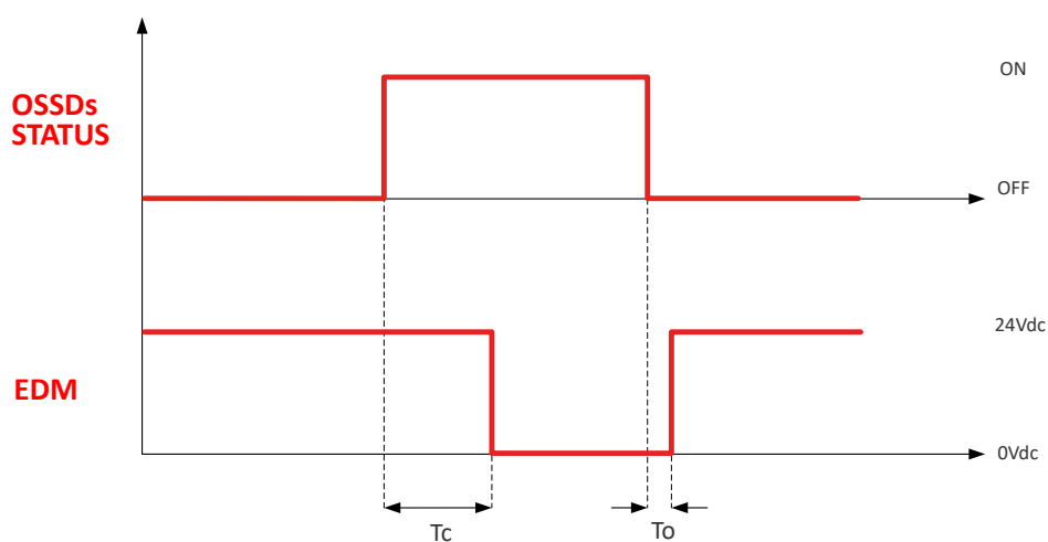
Figure 34 EDM function timing
