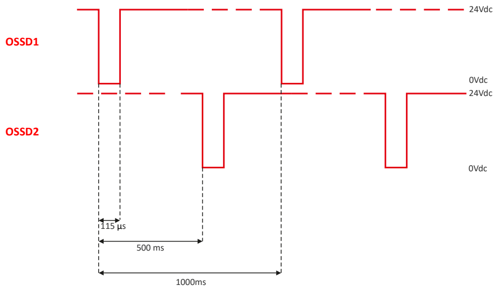
Figure 26: Behavior of OSSDs
