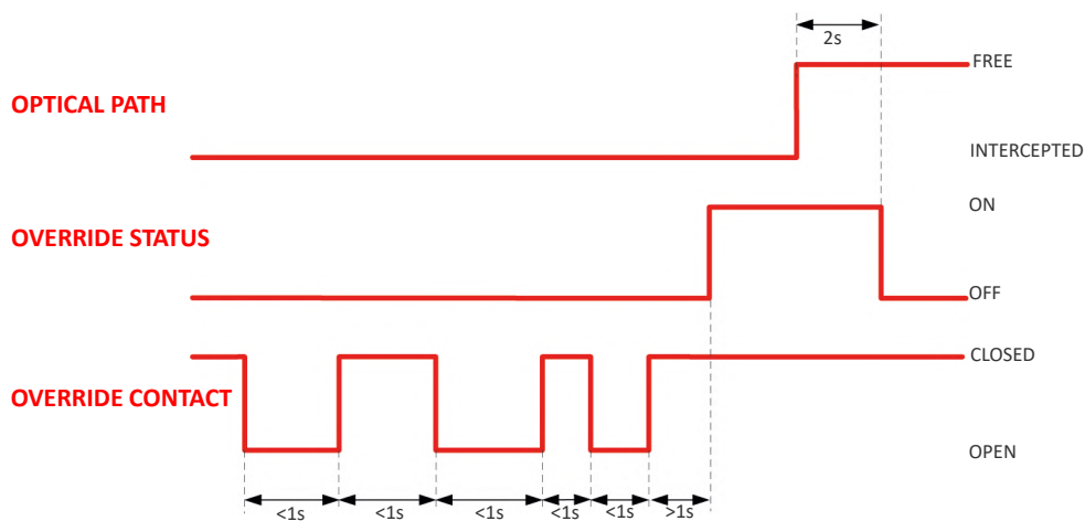
Figure 51: Override at Runtime timings
