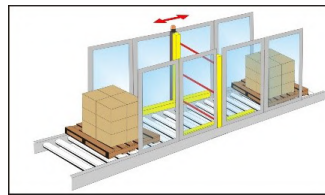
Figure 38: T-shaped version with integrated Muting sensors for bidirectional Muting
