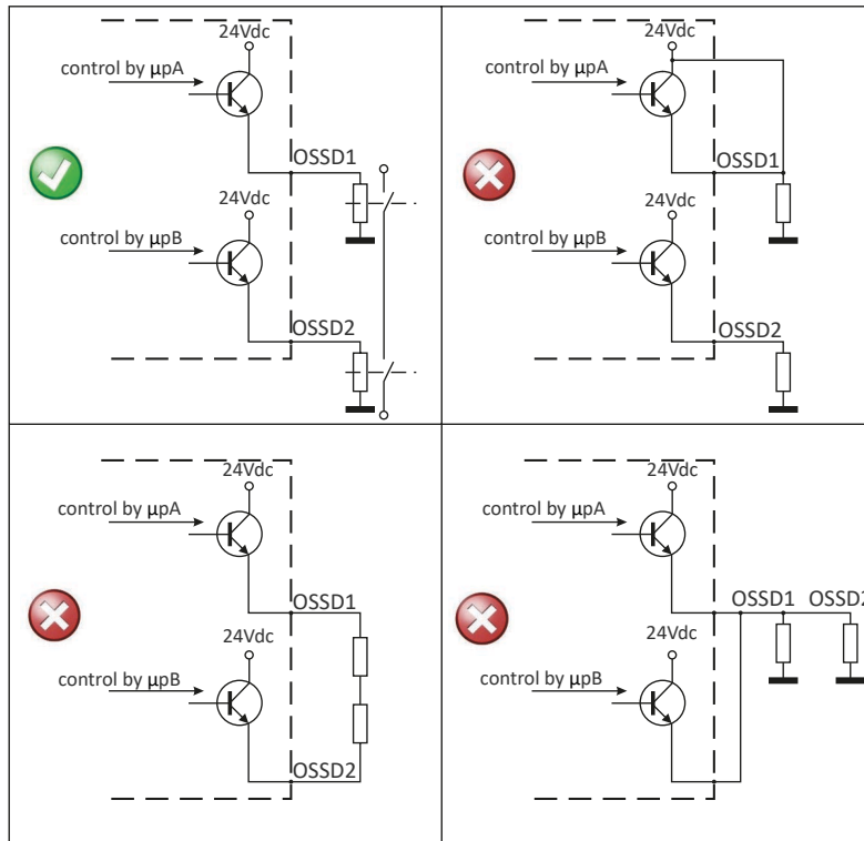
Figure 25: OSSDs connection
