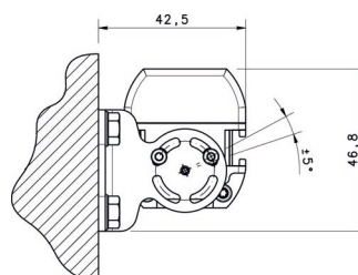
Figure 66 - Rotating 90° mounting
