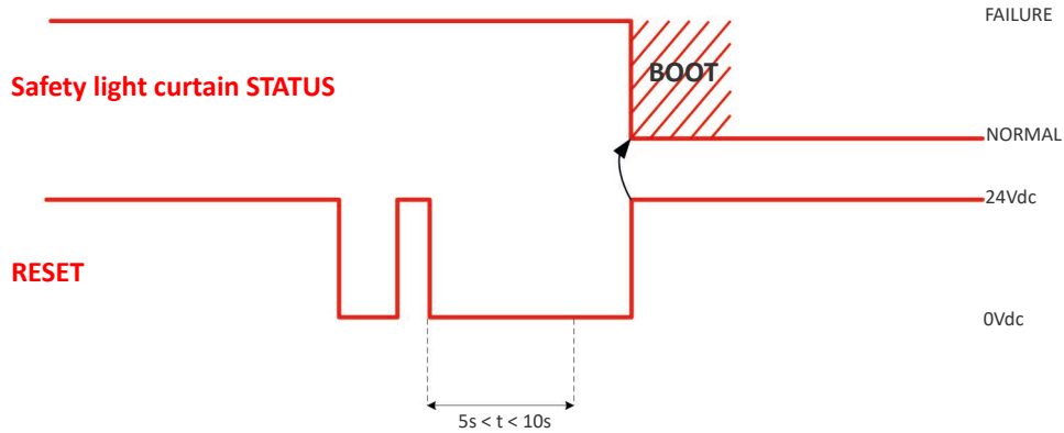
Figure 31: Reset function timing (SM-8)
