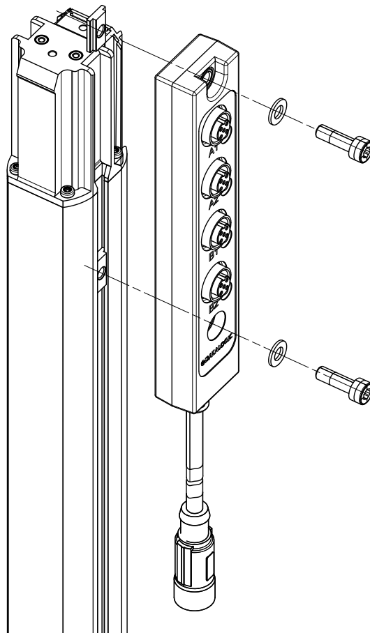
Figure 86 - Connection box
