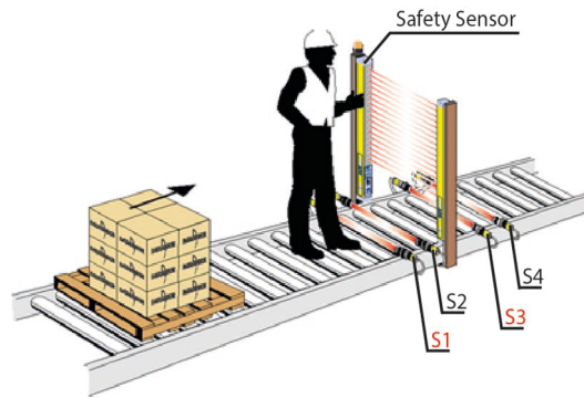
Figure 40: Typical Muting Application
