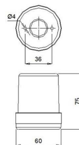
Figure 80: Lamp LMS-2
