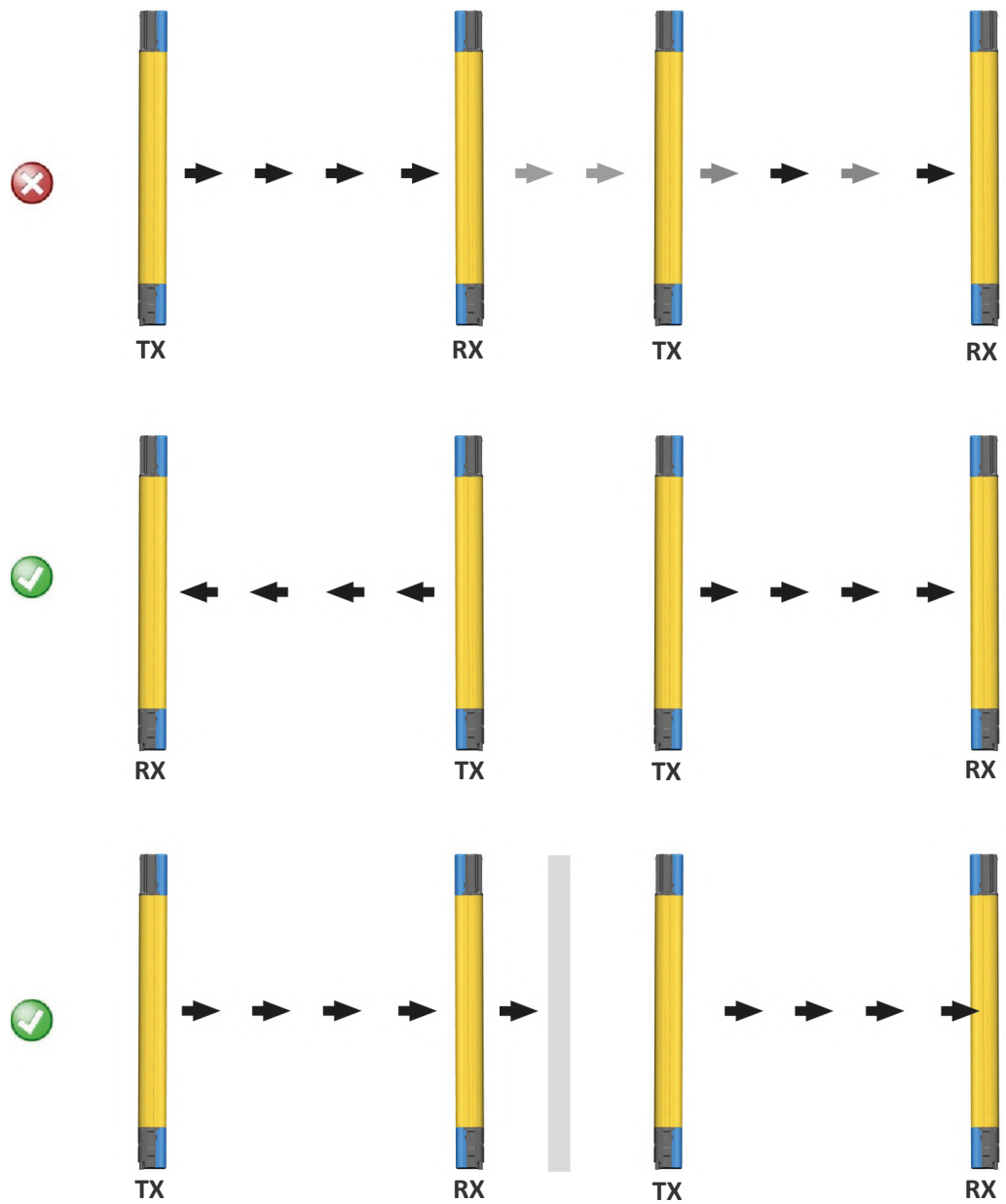
Figure 13: Recommended positioning for homologous devices
