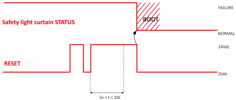
Figure 32: Reset function timing (SM-8-5)
