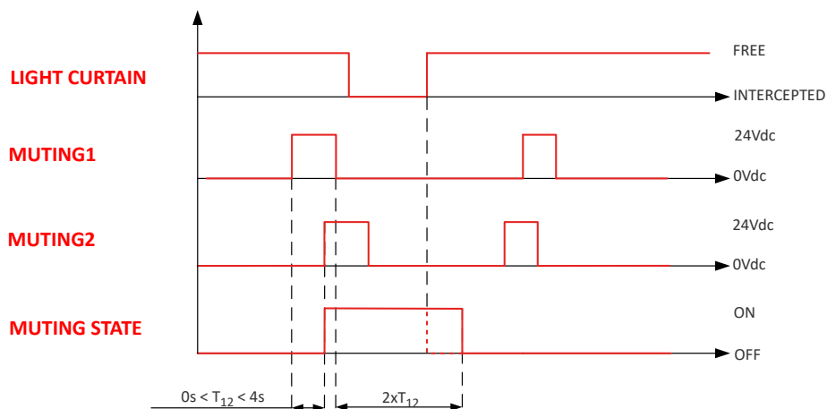
Figure 41: L muting timings
