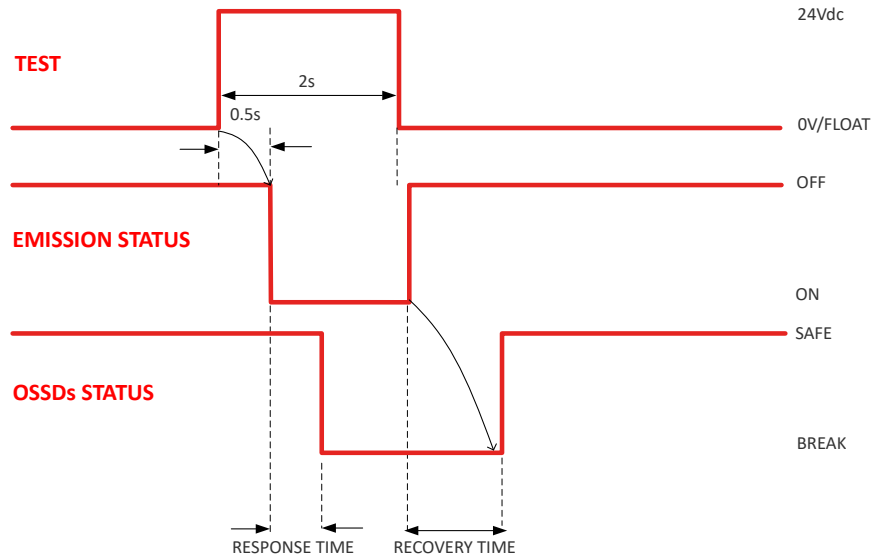
Figure 35 OSSDs timing for test on TX
