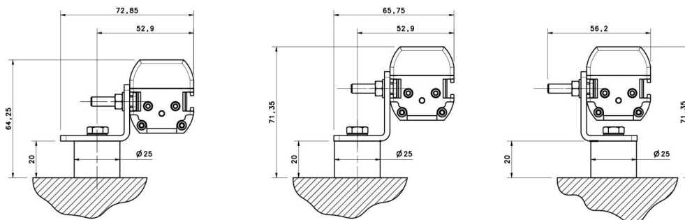
Figure 62 - Angled fixing bracket + Anti-vibration support
