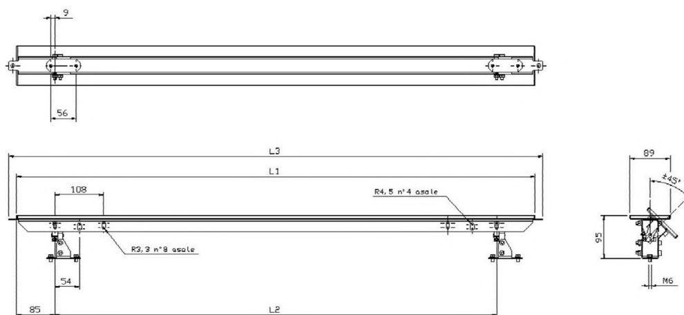
Figure 72 - Deviating mirrors (mm)
