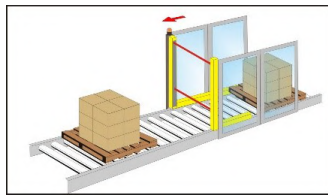
Figure 37: L-shaped version with integrated Muting sensors for unidirectional Muting
