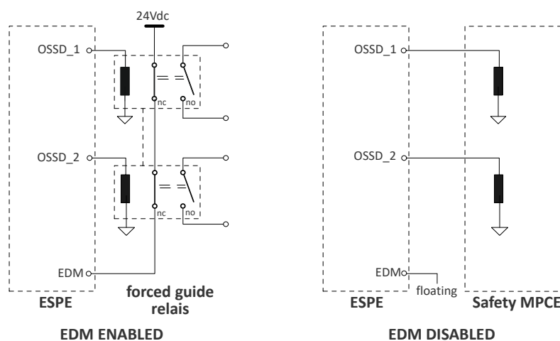
Figure 33: EDM wiring
