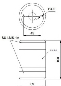
Figure 82: Module SU-LMS-1A + LMS-1
