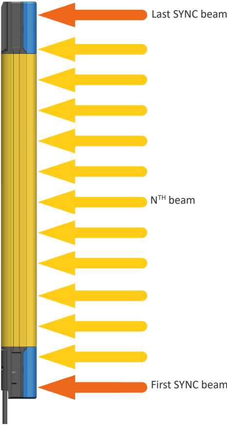
Figure 27: Description of the beams
