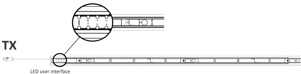
Figure 55: Transmitter LED interface
