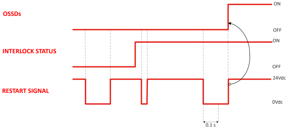
Figure 29: OSSDs behavior in Manual Restart Mode and Restart Pattern (SM-8)
