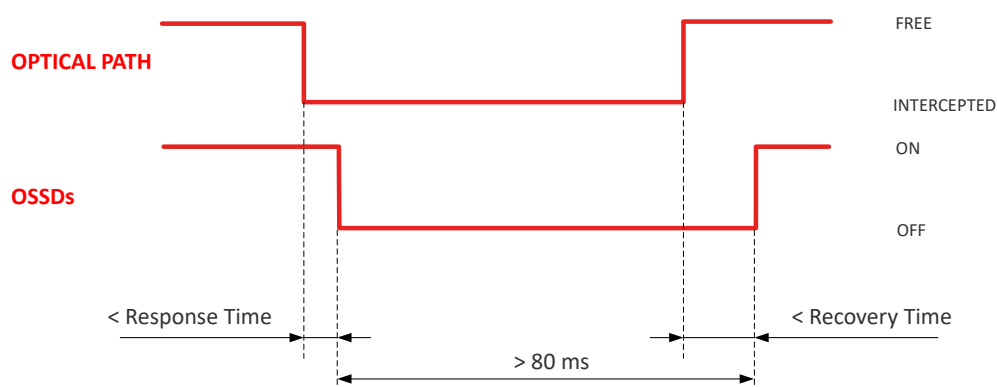
Figure 28: OSSDs behavior in Automatic Restart mode
