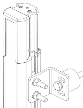
Figure 22: Anti-vibration dampers
