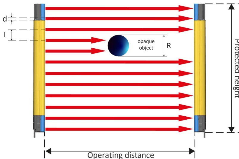
Figure 1: Detection capability
