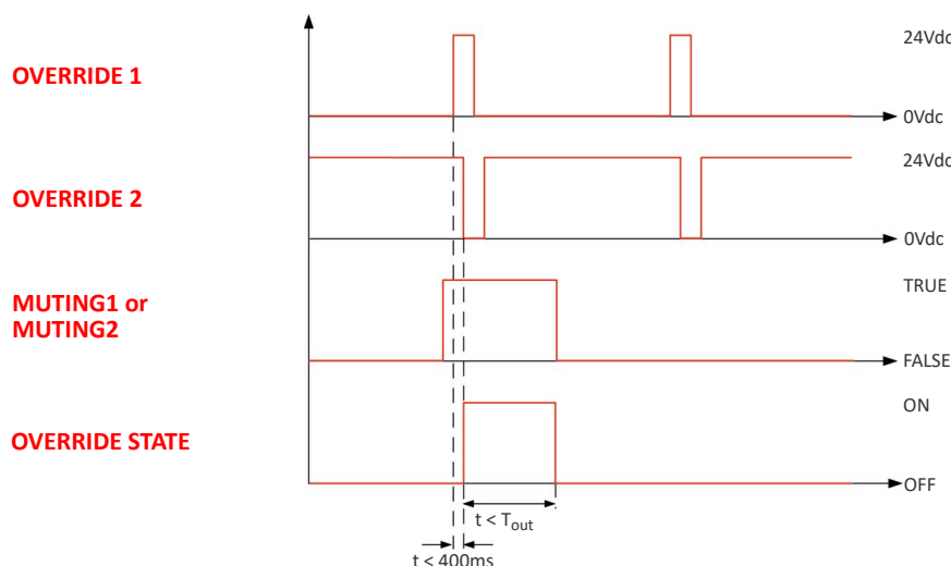
Figure 49: Edge Triggered Override Timings
