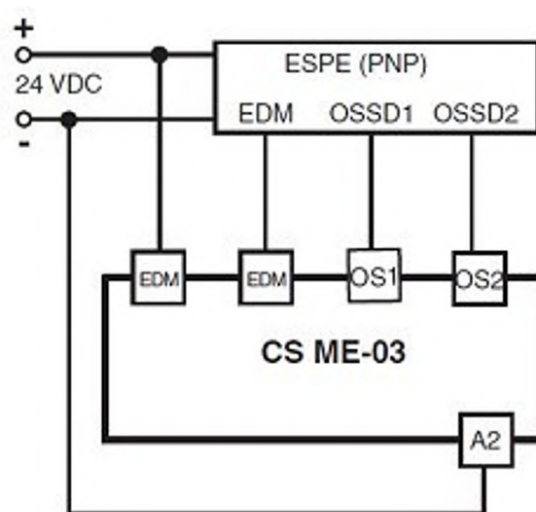
Figure 78 - EDM relay
