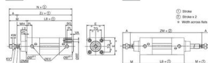
DIMENSIONS (mm), WEIGHT (kg) SINGLE-ROD TYPE CYLINDER Bare cylinder ISO 15552
