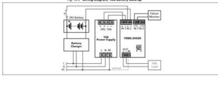
Fig. 18-3 Wiring diagram, 10A Battery back-up
