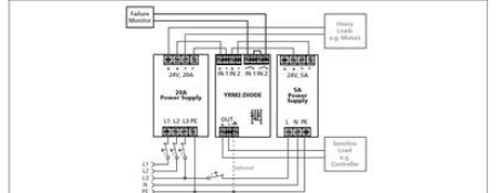
Fig. 18-4 Wiring diagram, redundancy for sensitive loads
