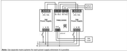
Fig. 18-1 Wiring diagram, 1+1 Redundancy, 10A output current
