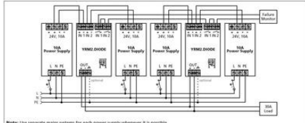
Fig. 18-2 Wiring diagram, n+1 Redundancy, 30A output current
