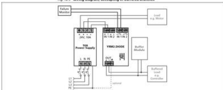
Fig. 18-5 Wiring diagram, decoupling of buffered branches
