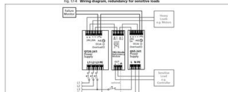
Fig. 17.4 Wiring diagram, redundancy for sensitive loads
