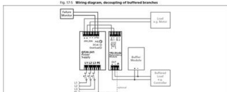
Fig. 17.5 Wiring diagram, decoupling of buffered branches
