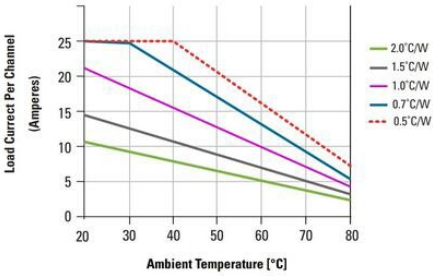
DERATE CURVES: 53TP IP20 25A
