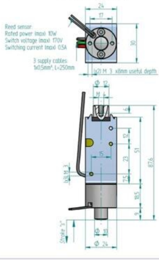
Solenoid locked
