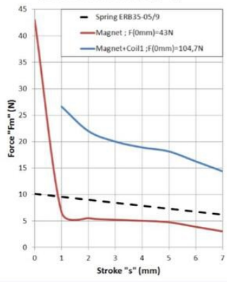
Force-stroke curve(F-S)
