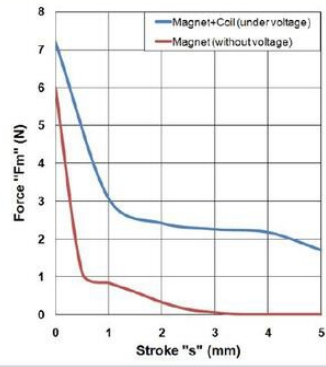
Force-stroke Curve (F-S)
