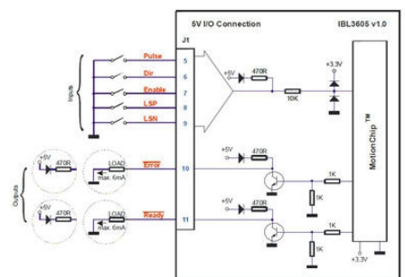
Figure 3.8. 5V Digital I/O connection
