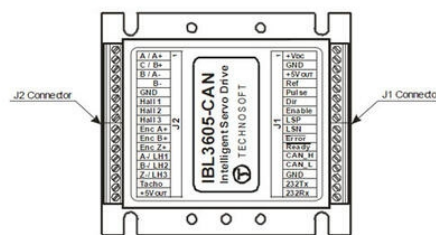
Figure 3.1. IBL3605 drive connectors
