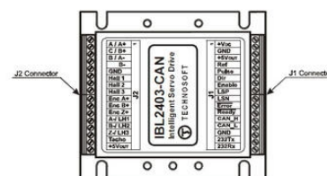
Figure 3.1. IBL2403 v1.1 drawing
