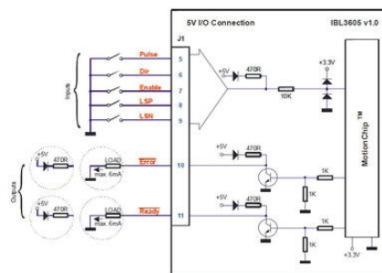
Figure 3.8. 5V Digital I/O connection
