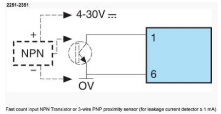
Fast count input NPN Transistor or 3-wire PNP proximity sensor (for leakage current detector \leq 1 mA)
