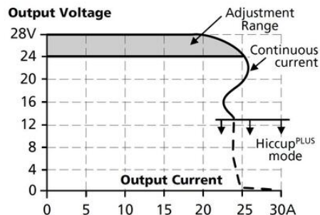
Output Voltage
