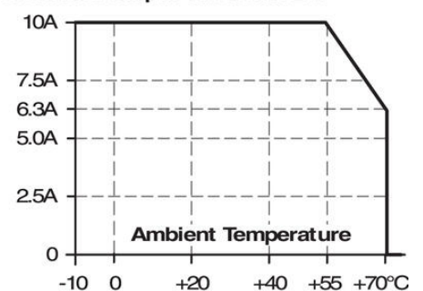
Allowable Output Current at 24V
