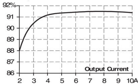
Efficiency
