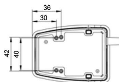
M3 BRASS FIXING INSERTS
