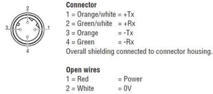
Camera EMOS Ethernet Front side of Molded M12-D 4p connector:
