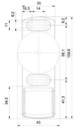
Anchor plate
