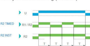
Function Di - Symmetrical flashing (ON Start)
